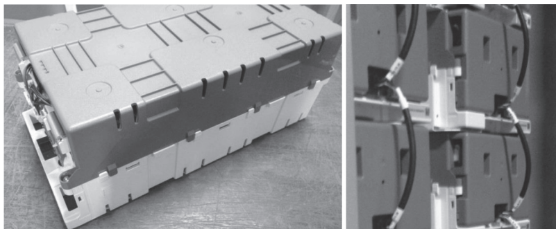
Figure 1 Li-ion battery module for 3-phase UPS applications (left) and multiple modules connected in a cabinet
