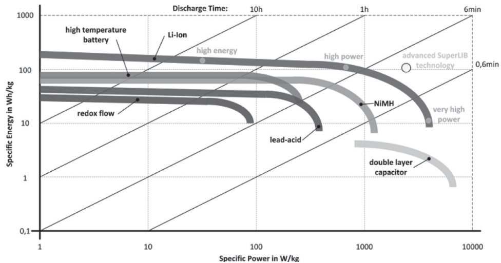
Figure 2 Chart showing relationship between energy and power density also known as a Ragone plot
